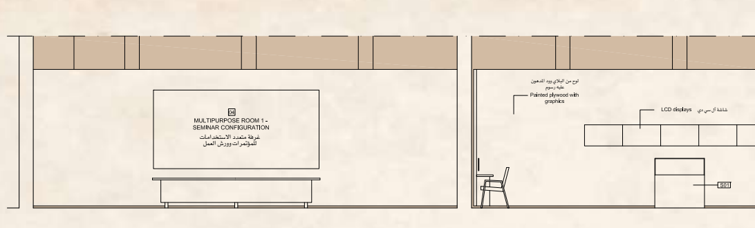
SECTION C-C' 1:50
